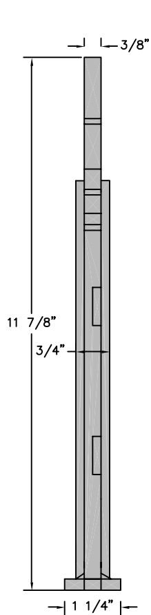
Plan View
