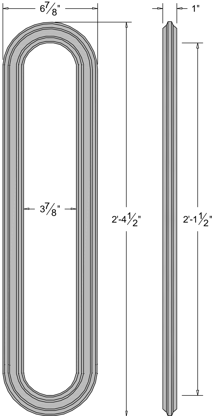
Front Elevation
