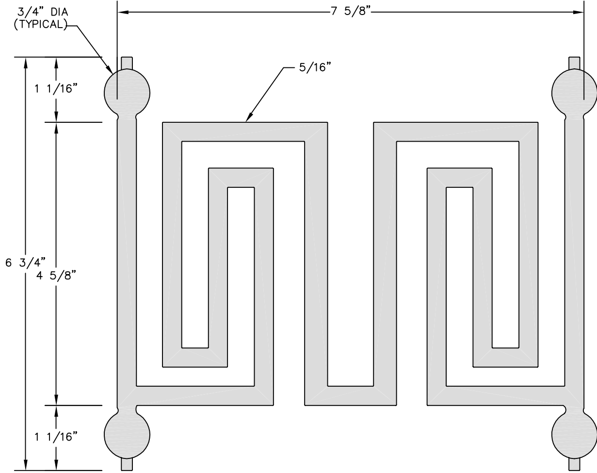
ELEVATION (FRONT & REAR SIMILAR)
