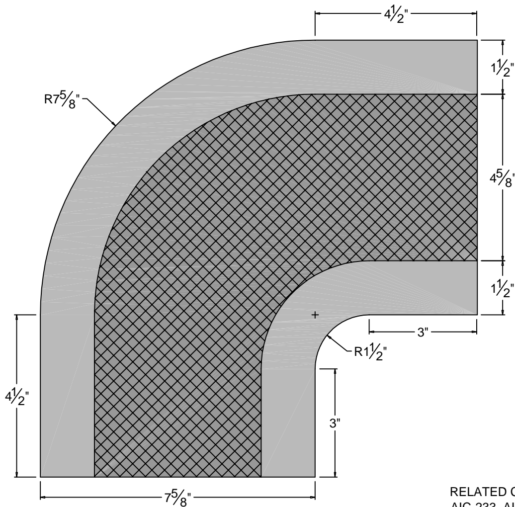
PLAN
