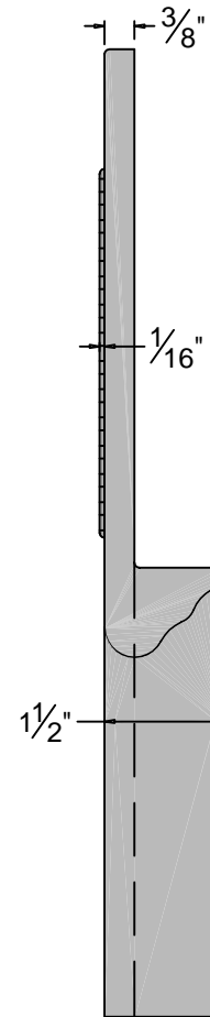
SIDE ELEVATION
