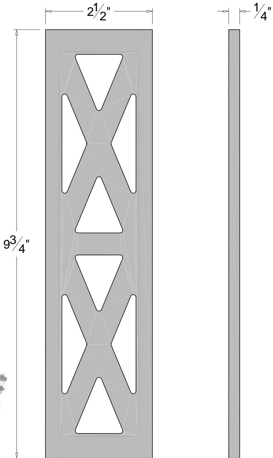
Front Elevation
