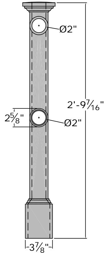
Front Elevation
