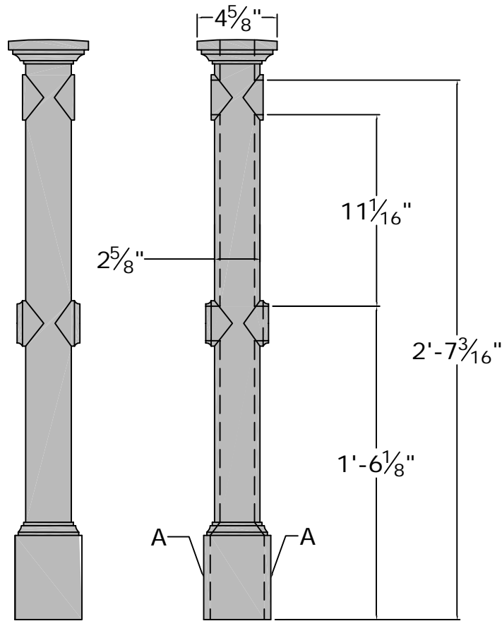
Plan Elevation
