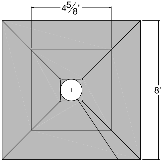
PLAN ELEVATION
