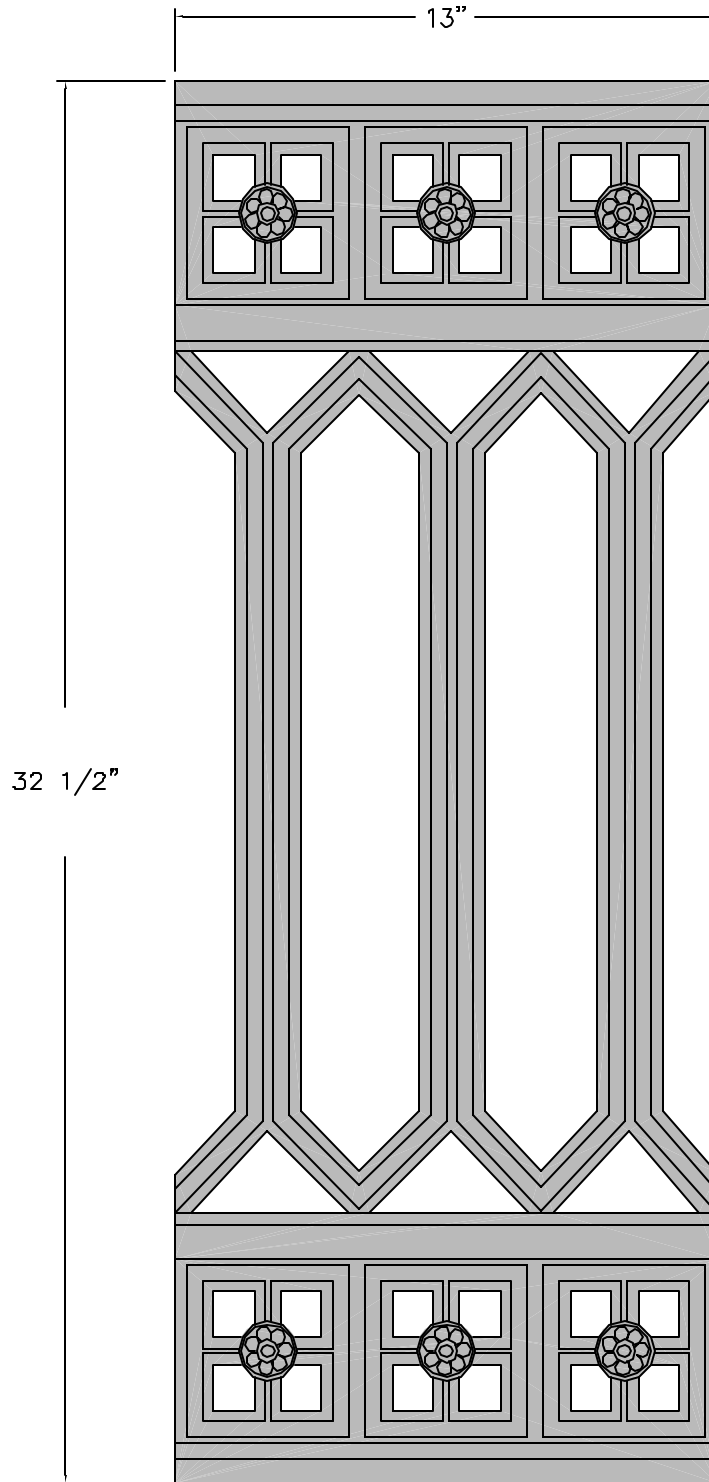
Front Elevation
