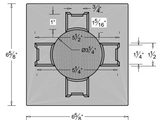
PLAN REFLECTED
