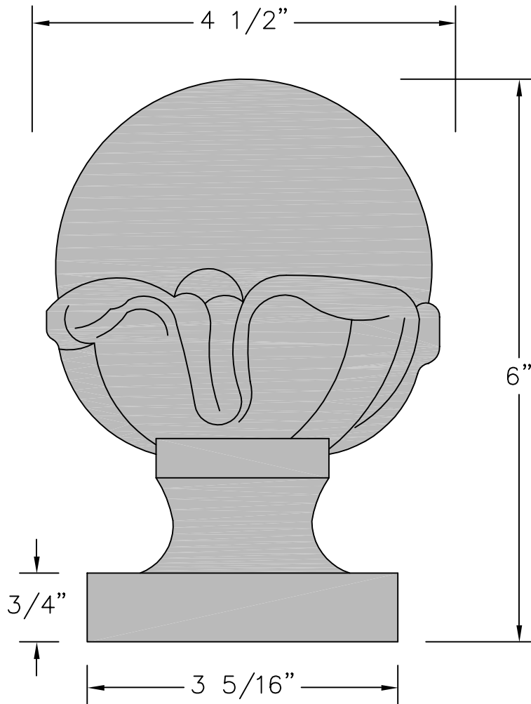
Side Elevation
