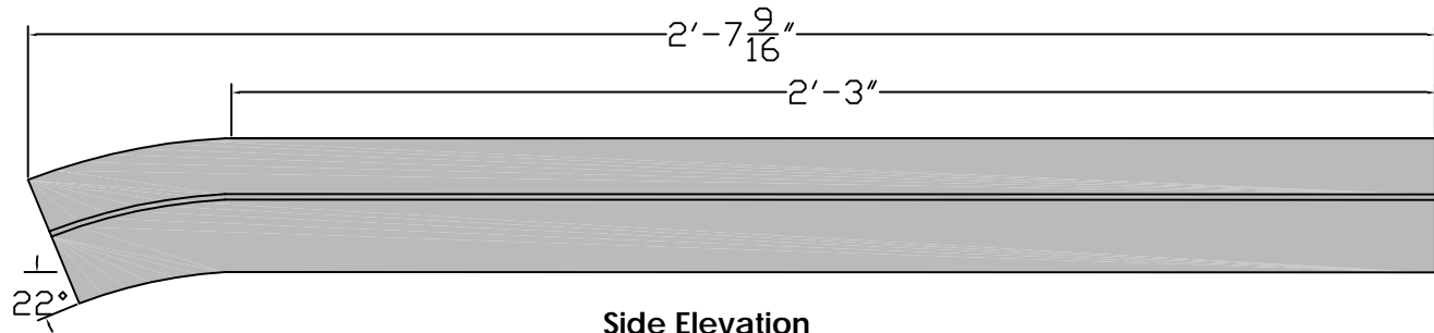
Side Elevation
