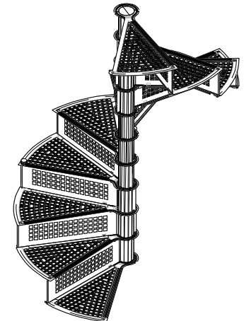
Partial Assembly
