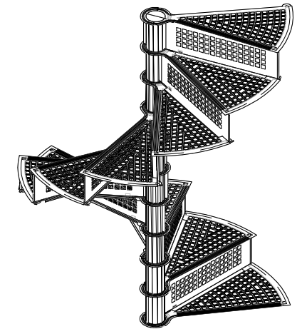
Partial Assembly
