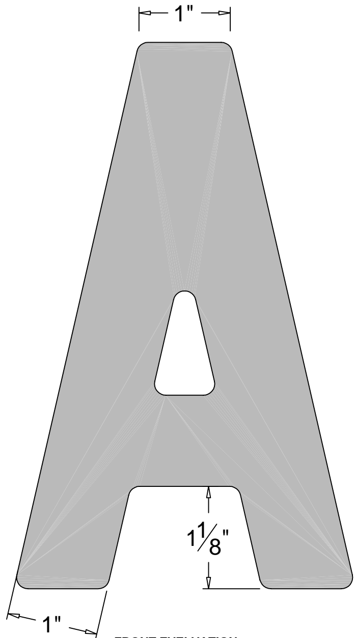
FRONT EVELVATION
