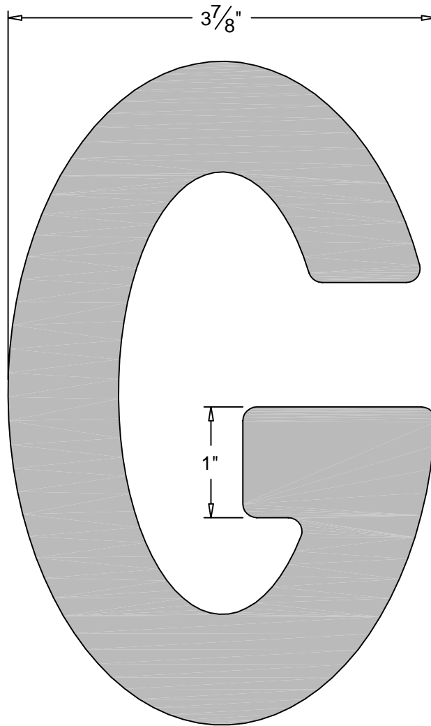
FRONT ELEVATION
