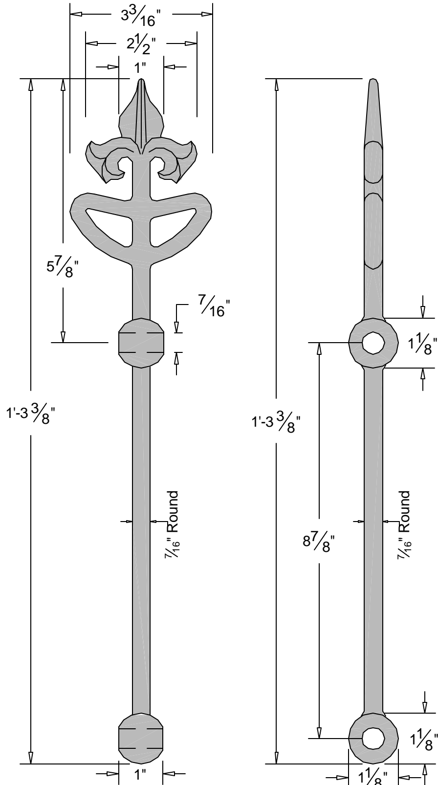
Front Elevation
