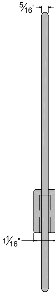
SIDE ELEVATION
