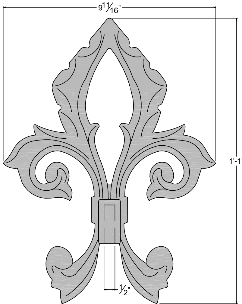
FRONT ELEVATION
