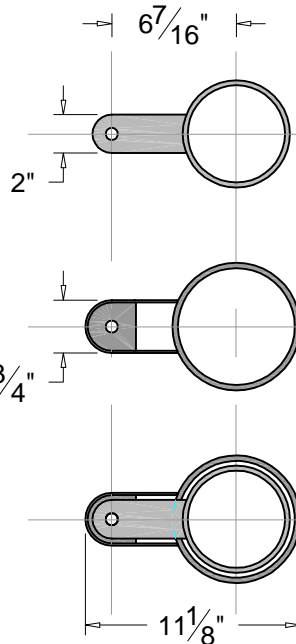
Detail: Bollard Plan at locking interface
