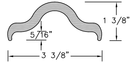
Handrail Section
